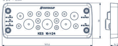
KES 16-1/24 2x Ø3.2 - 6.3mm 1x Ø4.0 - 7.5mm 1x Ø5.5 - 10.5mm 1x Ø8.0 - 12.5mm 1x Ø12 - 16.2mm
